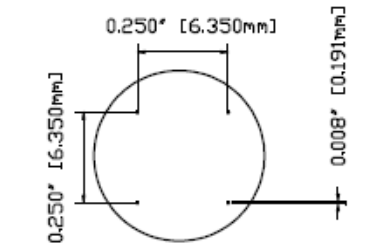
DETAIL A - DOT SPEC SCALE 5:1
