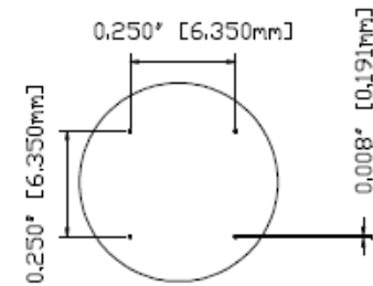
DETAIL A - DOT SPEC SCALE 5:1
