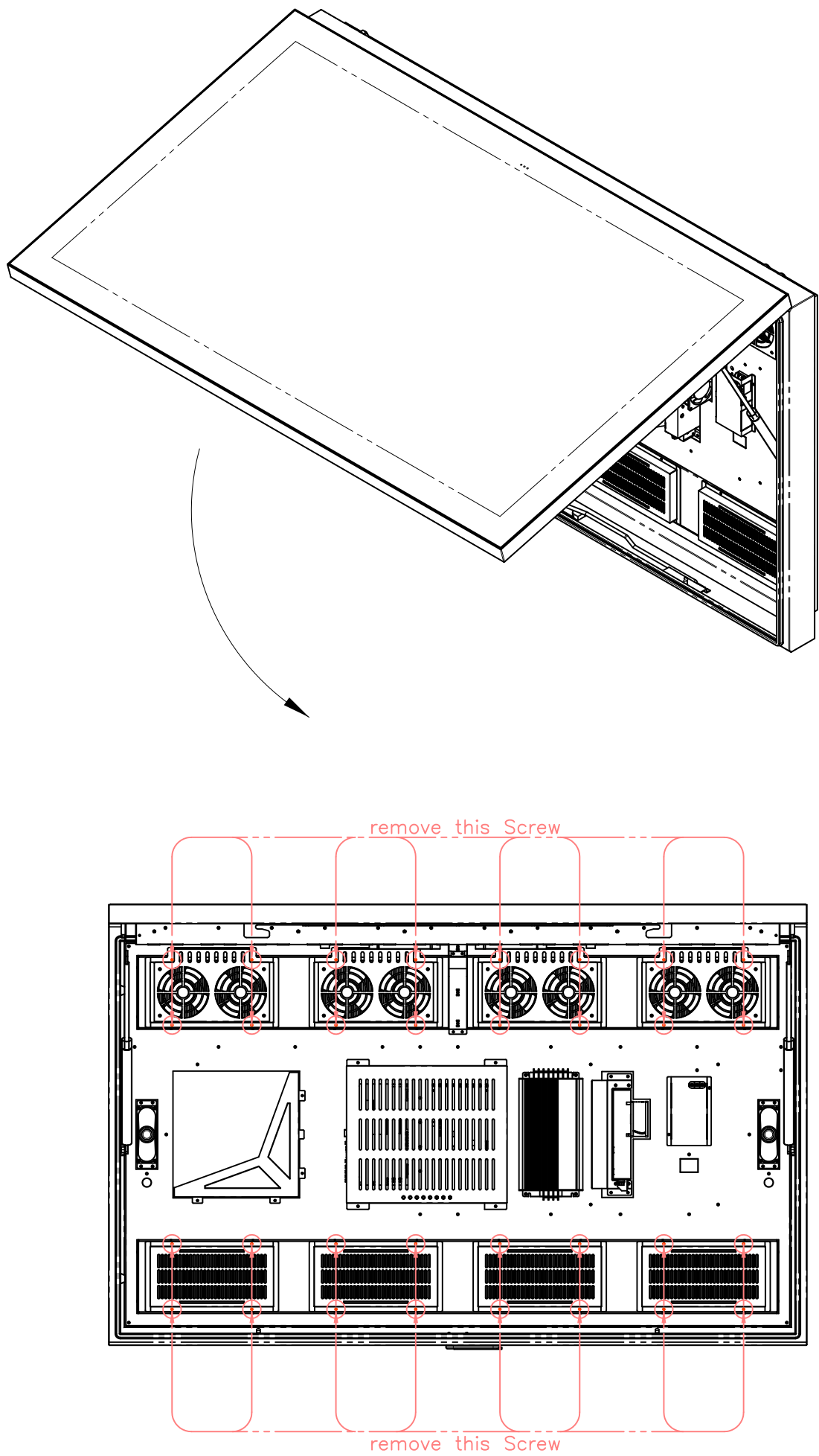
Front View (Door open)
