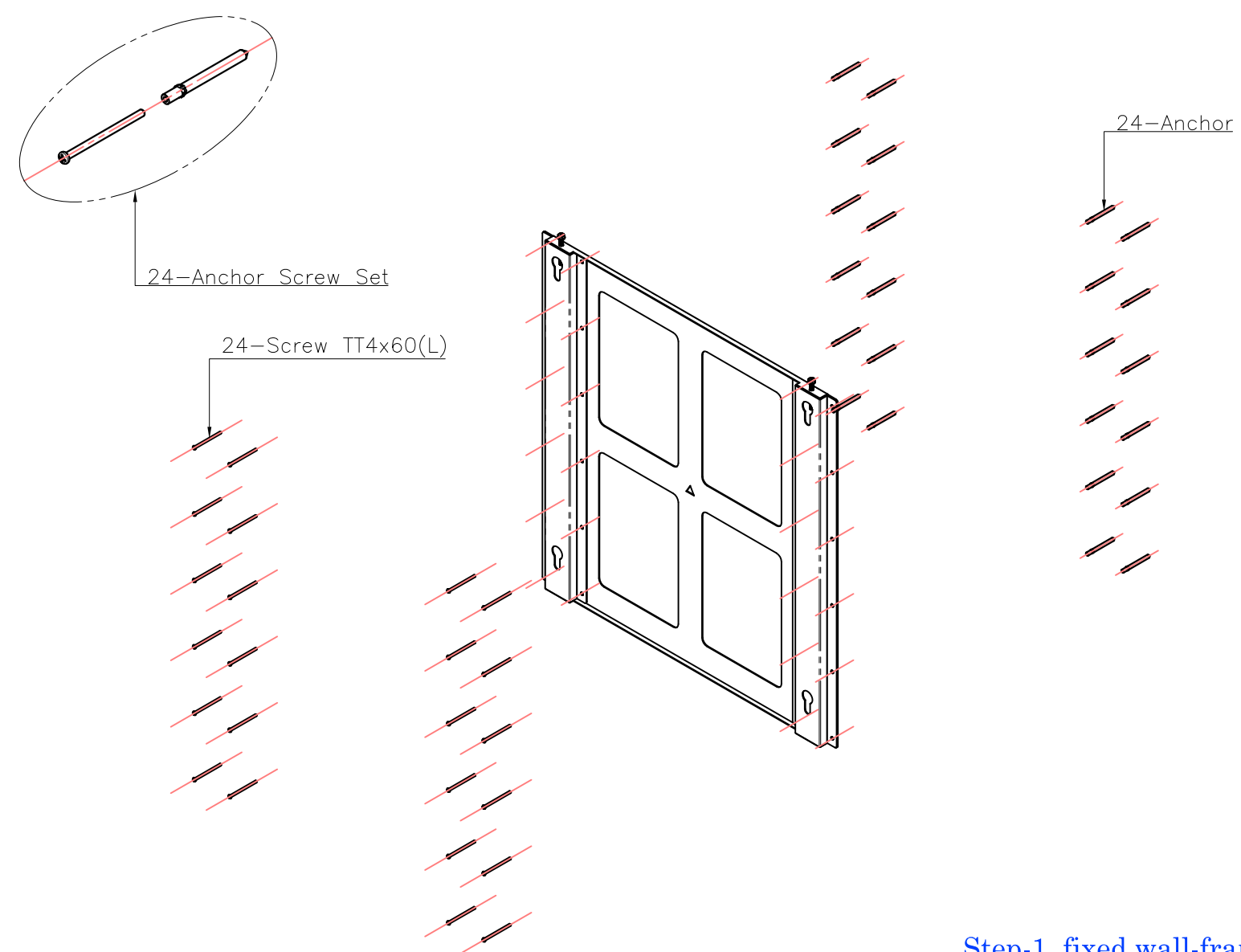
Step-1, fixed wall-frame
