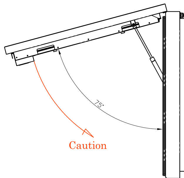
Side view (Right)
