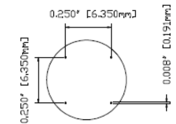
DETAIL A - DOT SPEC SCALE 5:1
